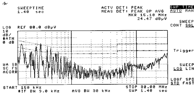
Plot 1. No external filter. Level B Quasi Peak and Average Limit-lines
