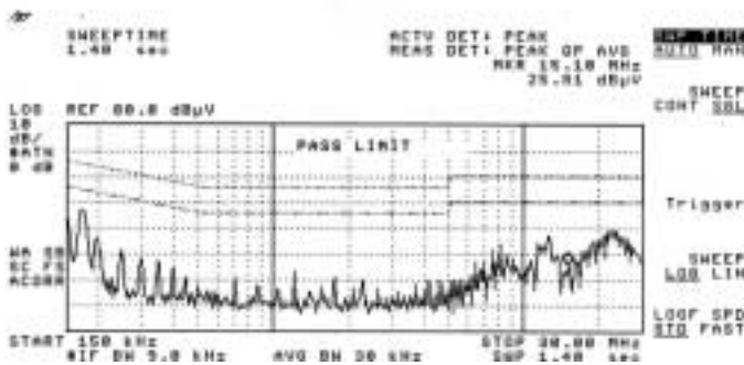
Plot 2. External filter as defined in AN105. Level B Quasi Peak and Average Limit-lines
